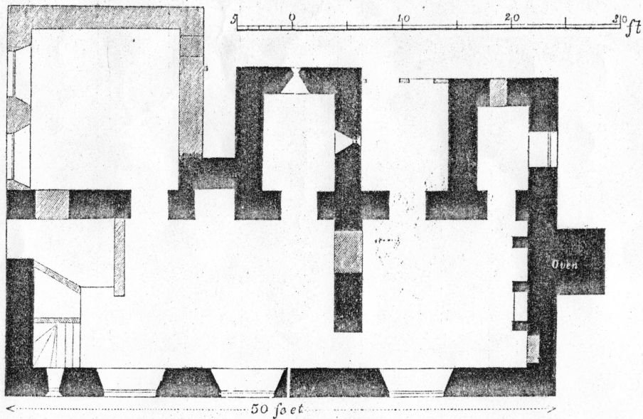
EAST FRONT PLAN OF MANOR HOUSE, COTTESFORD, OXFORDSHIRE.
